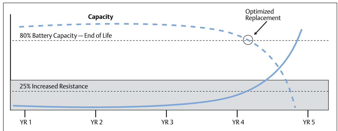
Figure 6. Batteries lose capacity as they age justifying the need for a preventive maintenance program.
