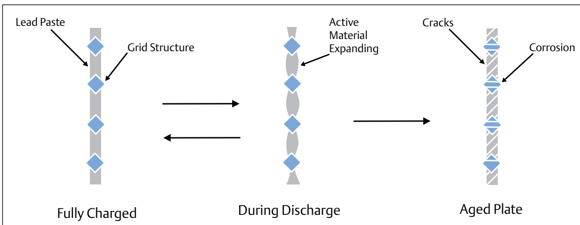
Figure 4. Illustrating mechanical stress. Grid does not shrink to 100 percent, which causes grid expansion.
