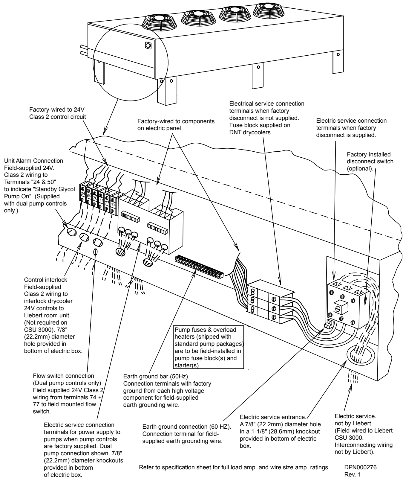
Figure 22 Electrical field connections for drycoolers with integral pump controls
