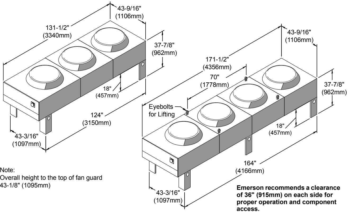
Figure 6 Drycooler planning dimensional data—Three- and four-fan units
