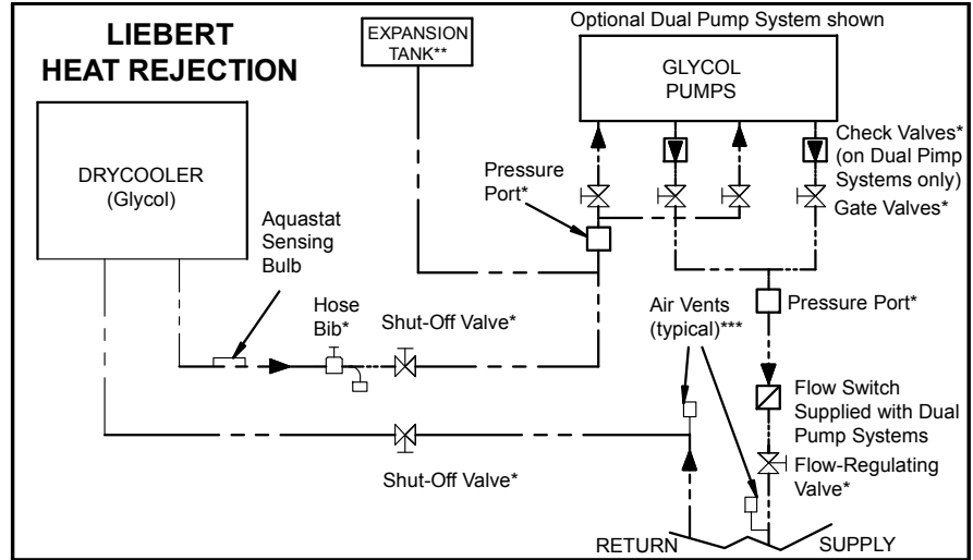
Figure 3 Piping diagram, Liebert DS with GLYCOOL with digital scroll compressors
