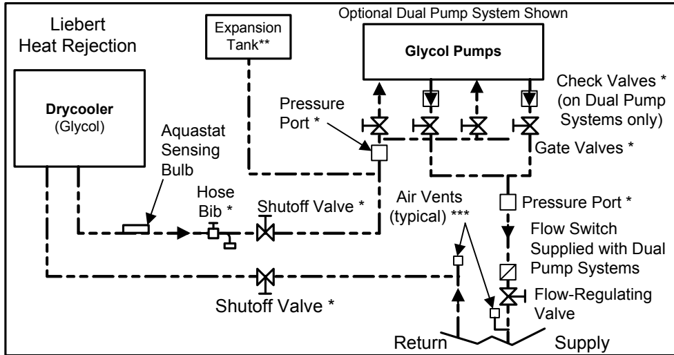
Figure 2 Piping diagram, Liebert DS glycol semi-hermetic compressor models
