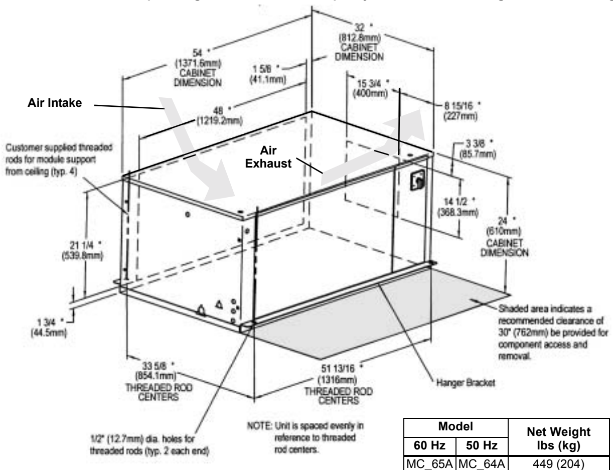
Figure 13 Cabinet and floor planning dimensional data—Split system—5-ton centrifugal fan condensing unit
