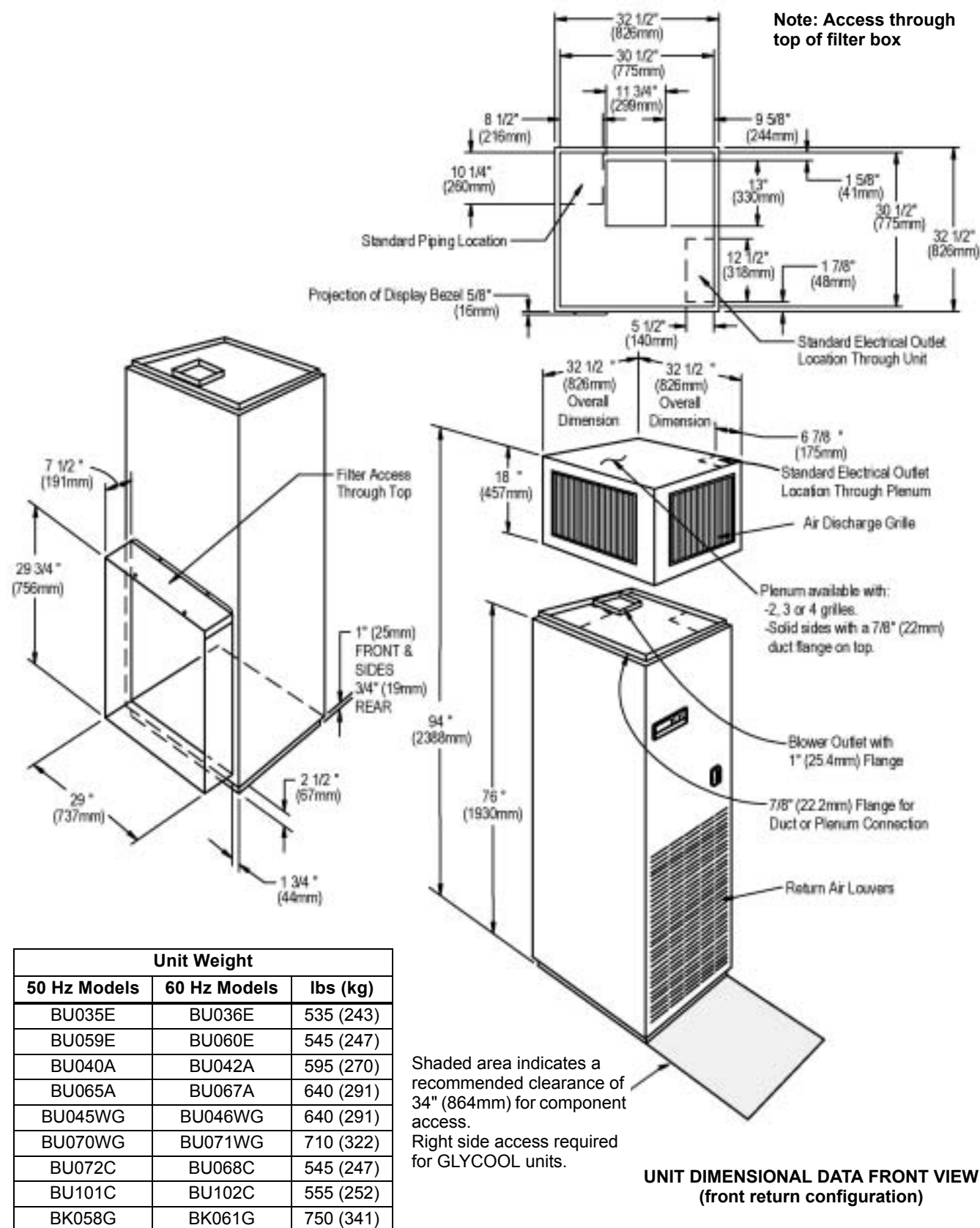
Figure 10 Cabinet and floor planning dimensional data—Upflow (BU/BK) models
