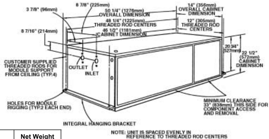
Figure 14 Cabinet and floor planning dimensional data—Split system—3-ton water/glycol cooled condensing unit
