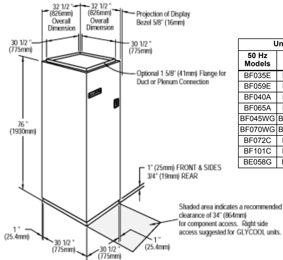
Figure 11 Cabinet and floor planning dimensional data—Downflow (BF/BE) models
