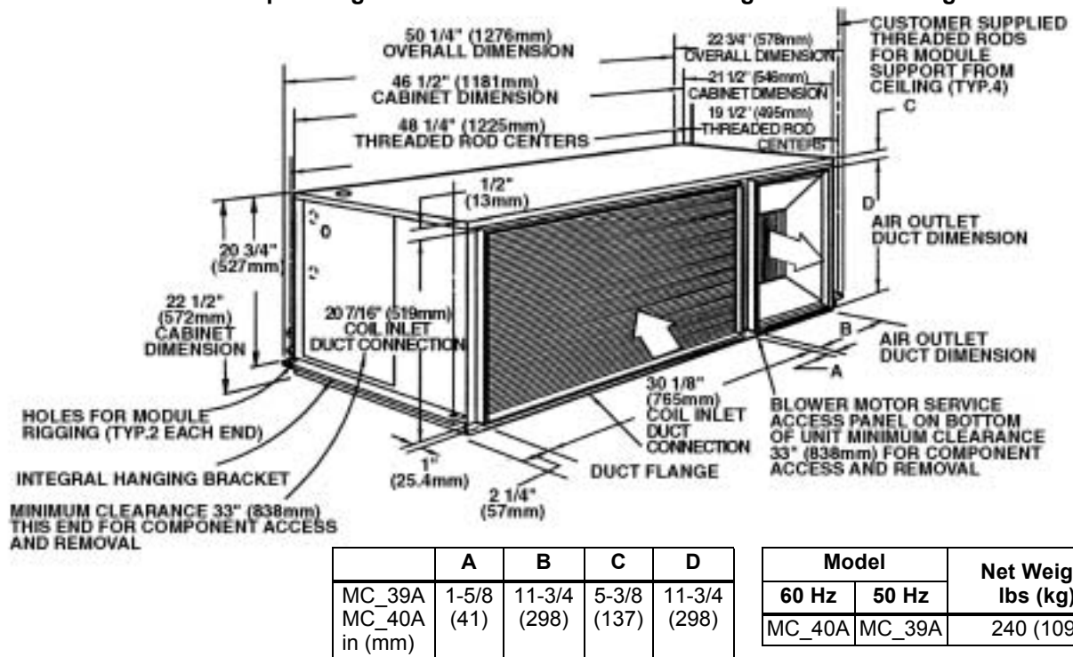
Figure 12 Cabinet and floor planning dimensional data—3-ton centrifugal fan condensing unit
