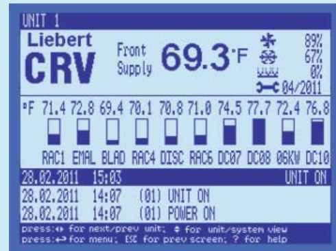
Bar graphs show the inlet temperature of every rack with a 2T temperature sensor.
